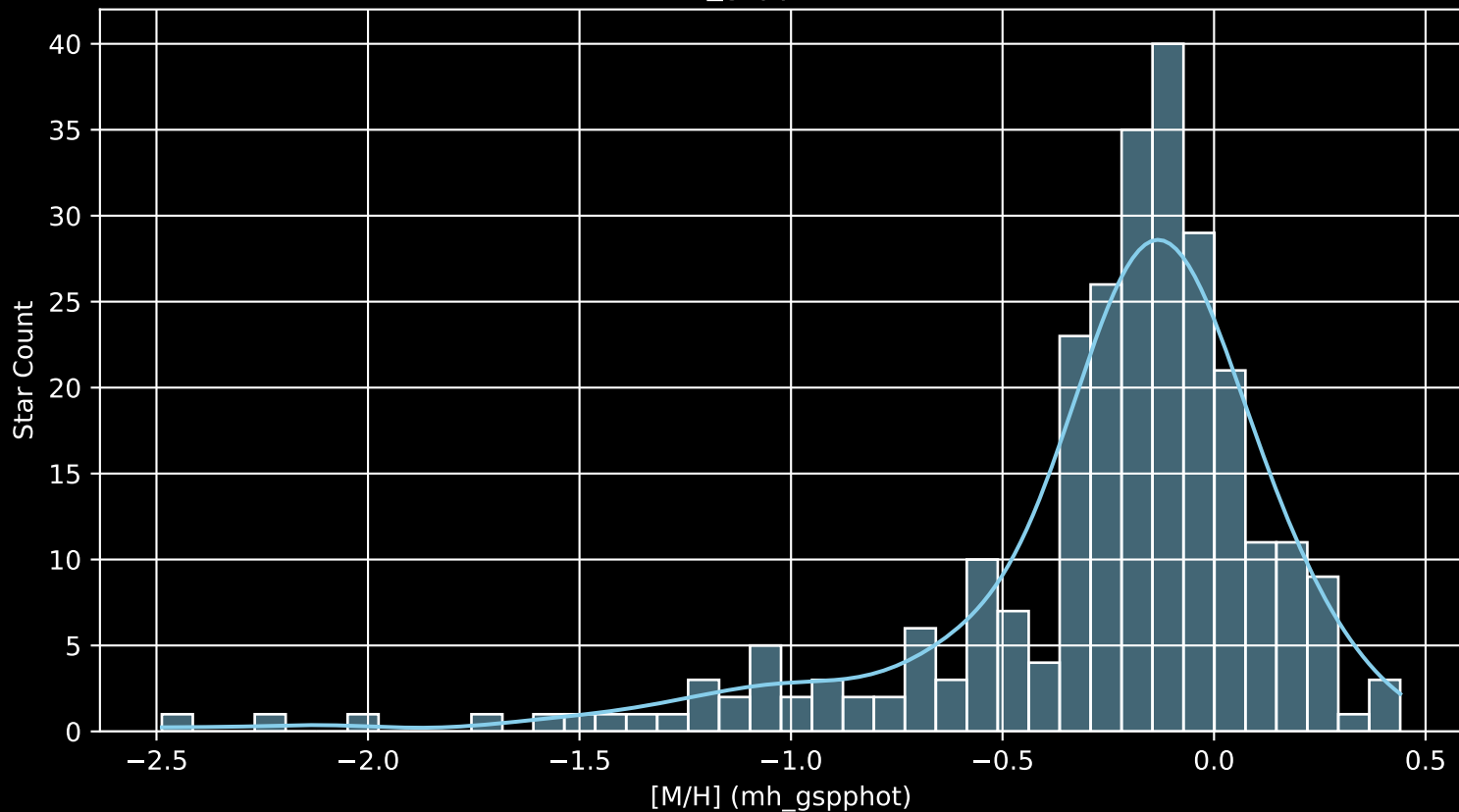
APOGEE DR17 Field: [139+00 [M/H] (mh_gspphot) (n= 267)
