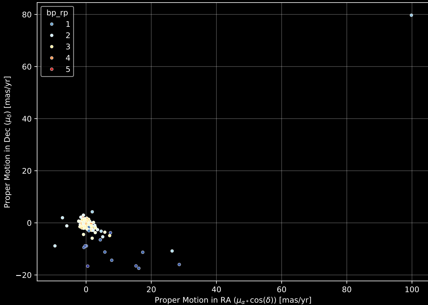
APOGEE DR17 Field: [139+00] Proper Motion Diagram (n= 271)
