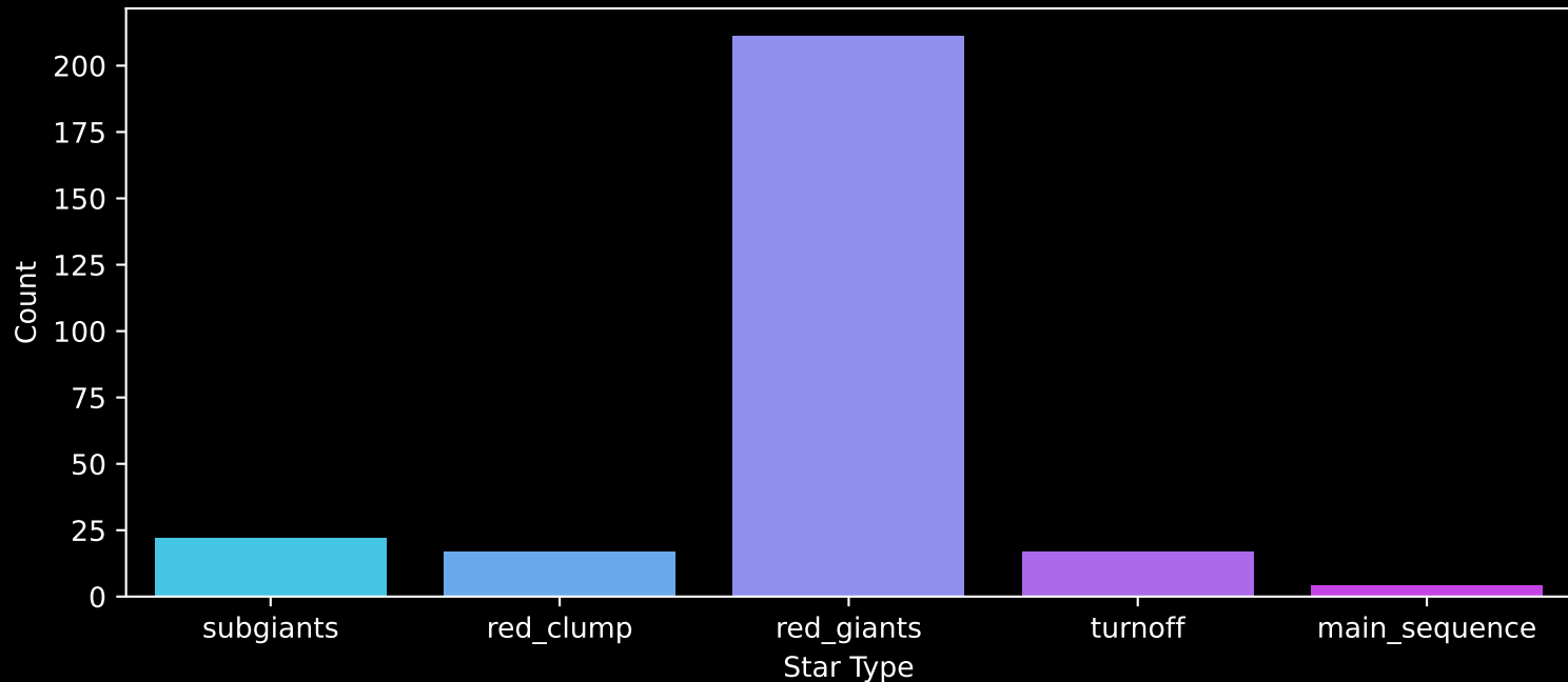
APOGEE DR17 Field: [139+00] Count plot of Star Type
