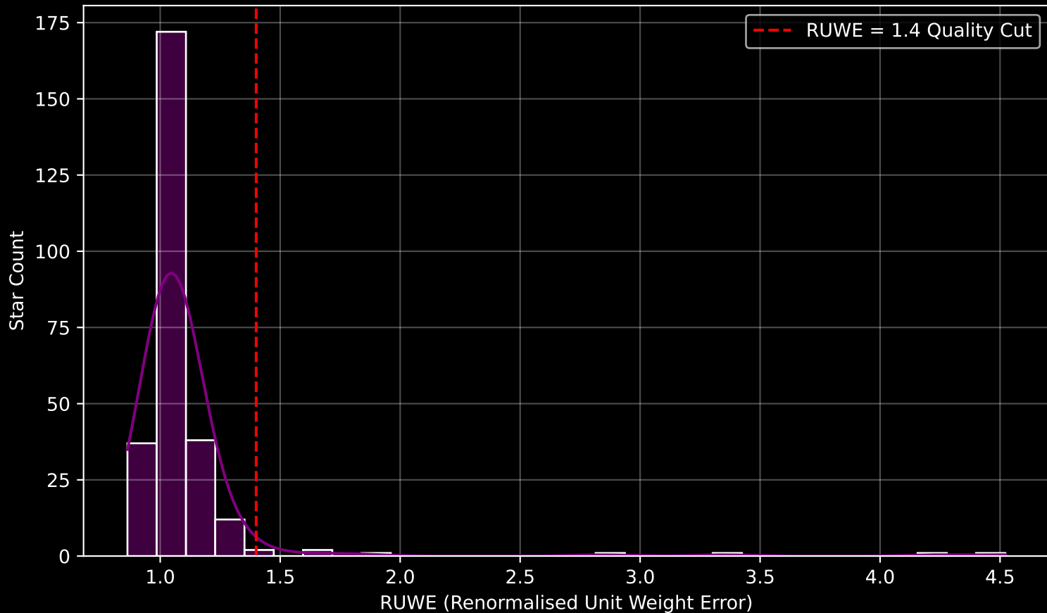
GAPOGEE DR17 Field [139+00] RUWE Distribution (n= 268)
