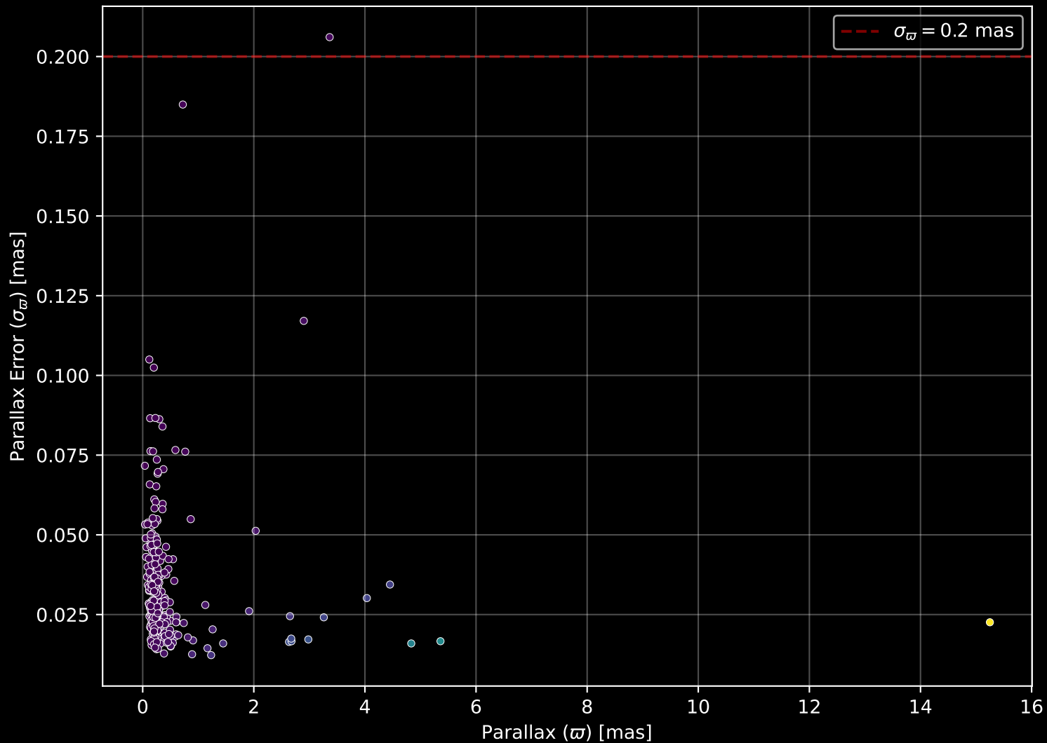
APOGEE DR17 Field: [139+00] Parallax Quality (n= 271)
